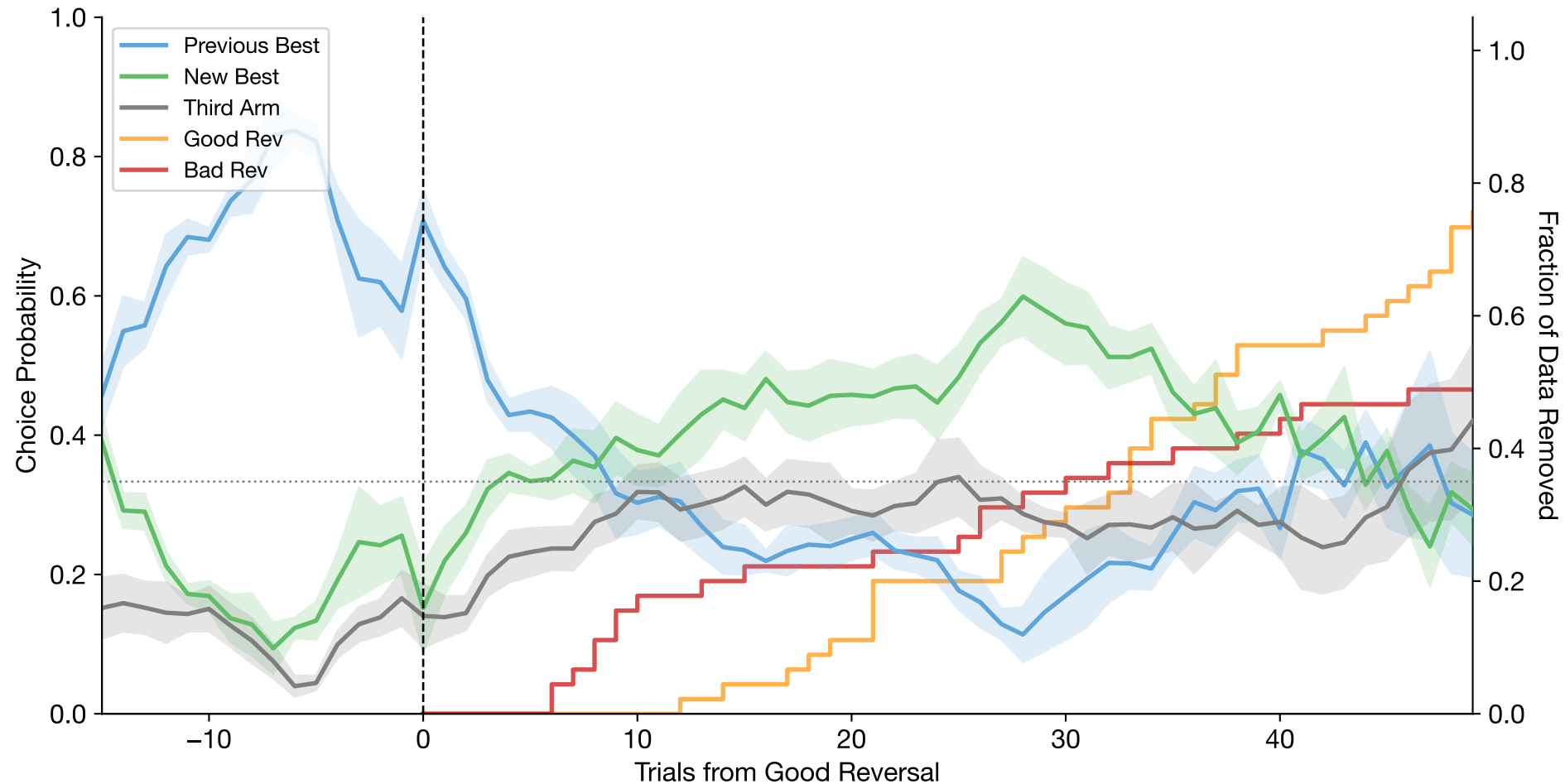
Good Reversal-Aligned Choices (mean \pm se across subjects | n=6 subjects, n=45 reversals)
